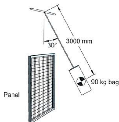
FIGURE E1 BARRER TEST METHOD
