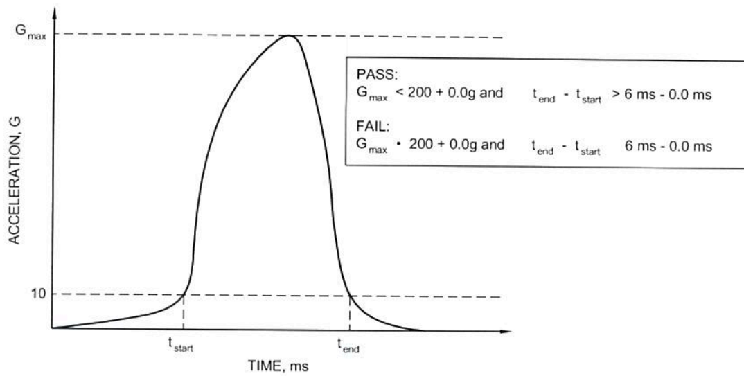
(a) Example of a single-peak acceleration impulse
