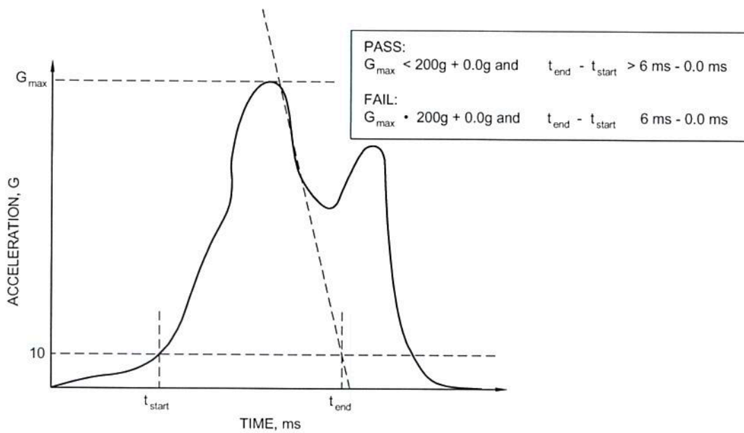
(b) Example of a multi-peak acceleration impulse
